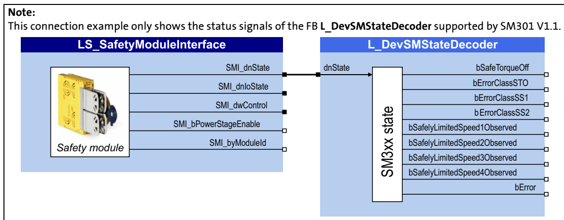
[2-1] Example: Decoding of the SMI_dnState status signal into individual boolean status signals
