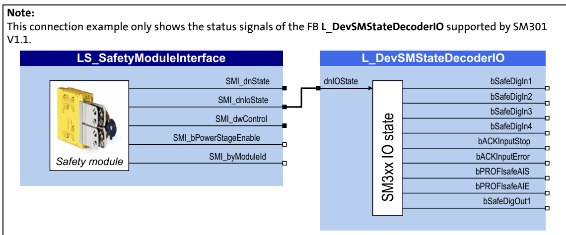
[2-2] Example: Decoding of the SMI_dnloState status signal into individual boolean status signals
